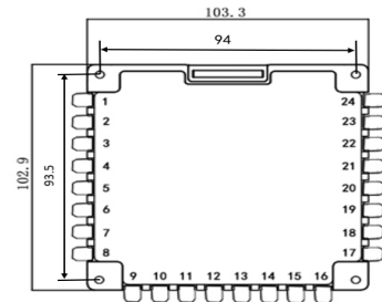
Mounting Hole \Phi 3.3mm
